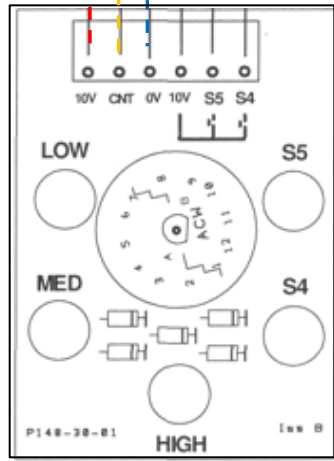
3-SPEED CONTROLLER
