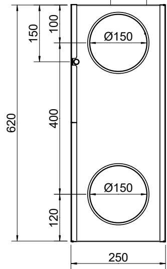
FRESH AIR END VIEW
