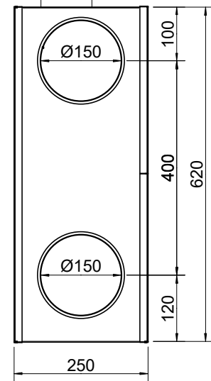
SUPPLY AIR END VIEW
