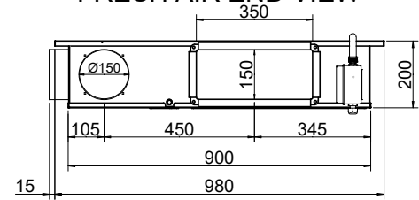
FRESH AIR END VIEW
