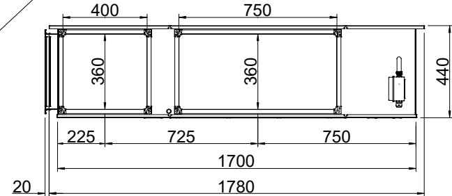
FRESH AIR END VIEW
