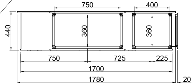
SUPPLY AIR END VIEW
